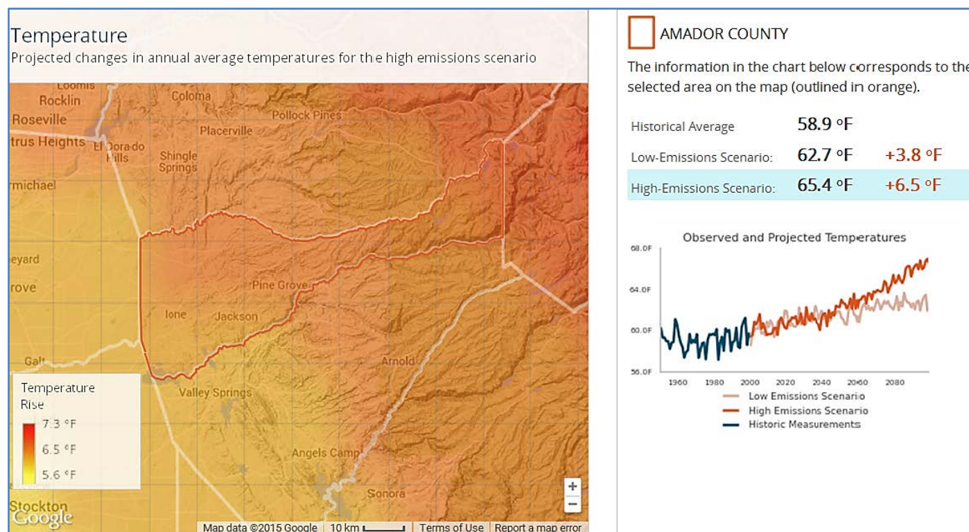
Figure 2. Projected changes in annual average temperature in future carbon emissions scenarios, Amador County, 2099 6
