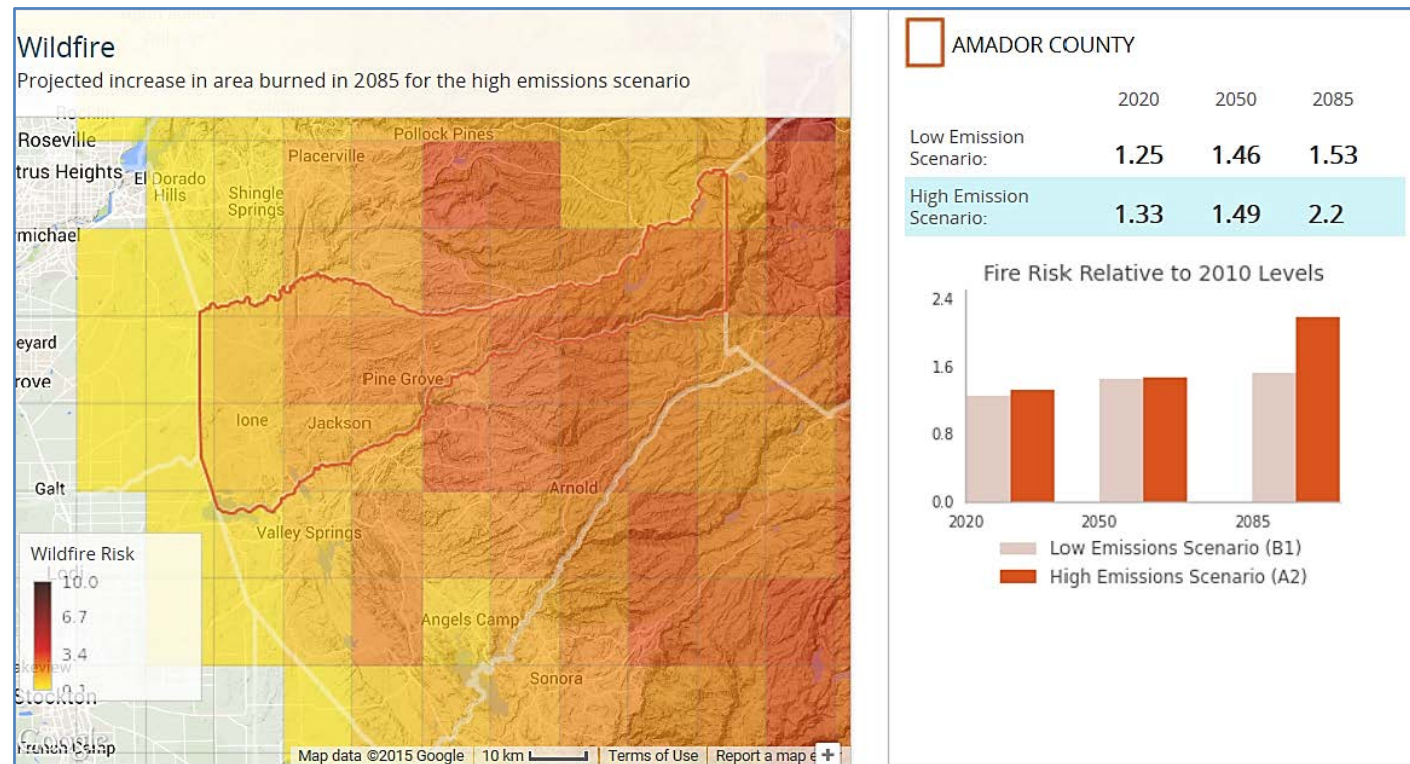
Figure 4. Relative increase in wildfire acreage in future carbon emission scenarios, Amador County 6
