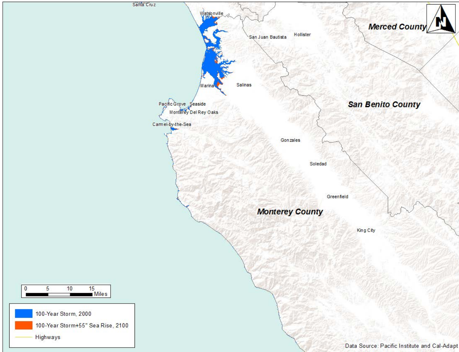
Figure 5. Baseline inundation areas for a 100-year flood (2000) and modeled scenario with additional 55 inches of sea level rise (2100), Monterey County 6 Note: Current projections are 66 inches above sea level. 7
