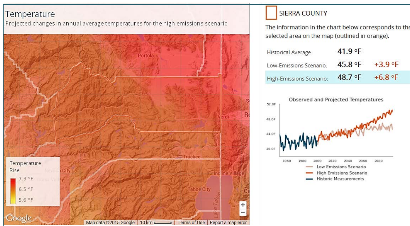
Figure 2. Projected changes in annual average temperature in future carbon emissions scenarios, Sierra County, 2099 6
