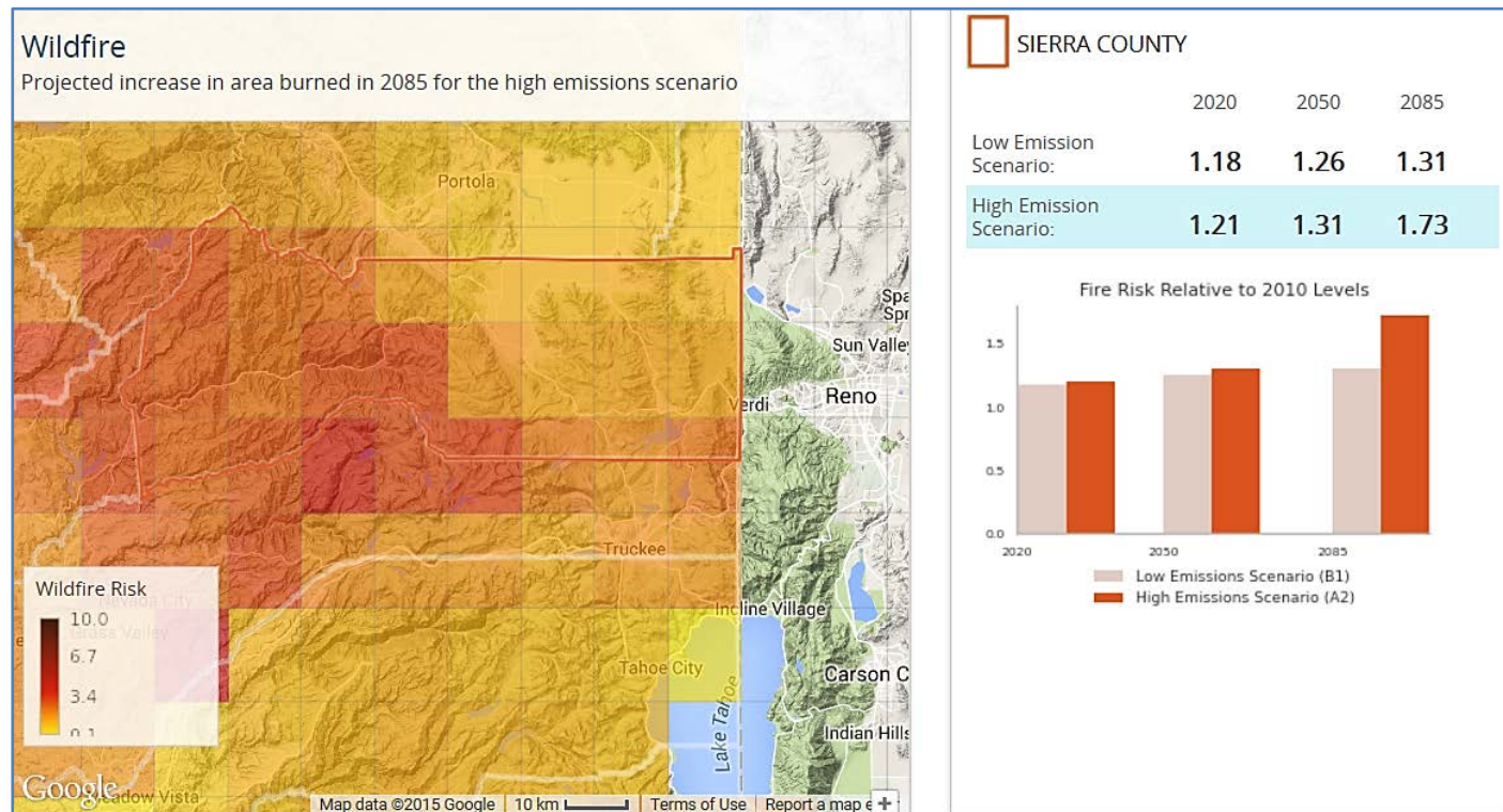
Figure 4. Relative increase in wildfire acreage in future carbon emission scenarios, Sierra County 6
