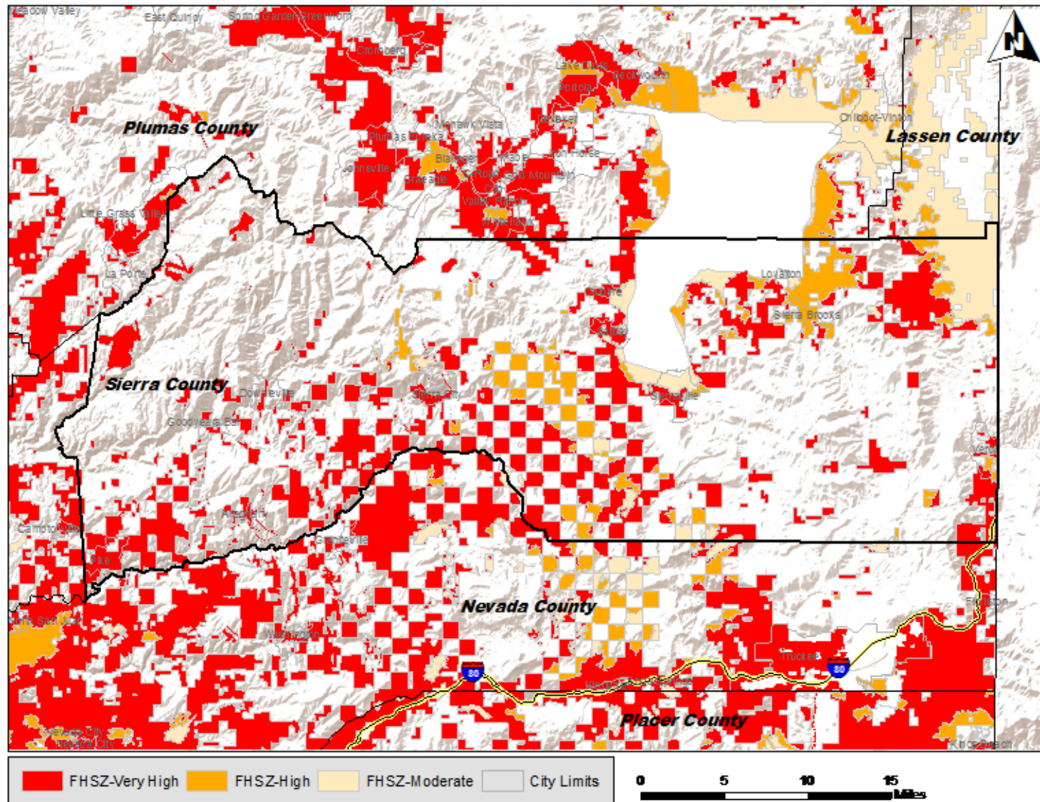
Figure 3. Current Fire Hazard Severity Zones (FHSZ), Sierra County, 2007 8
