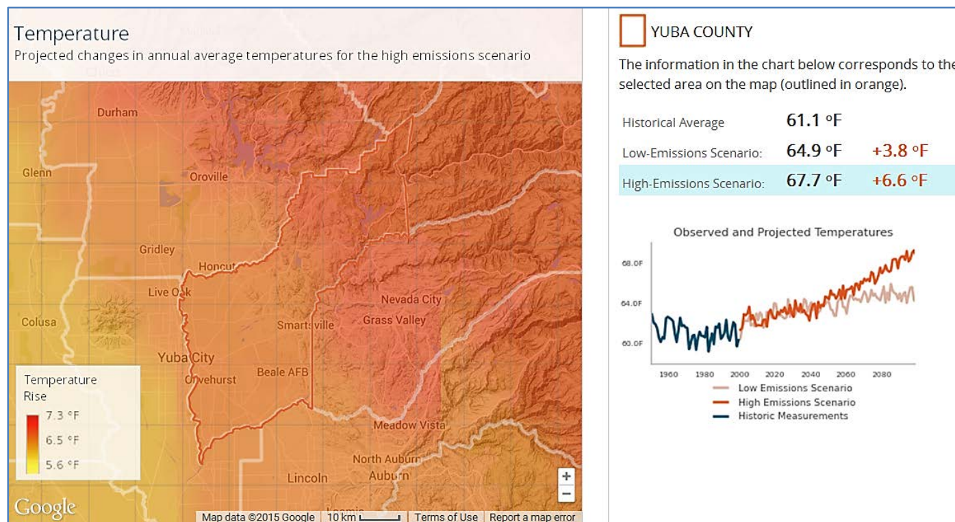
Figure 2. Projected changes in annual average temperature in future carbon emissions scenarios, Yuba County, 2099 6
