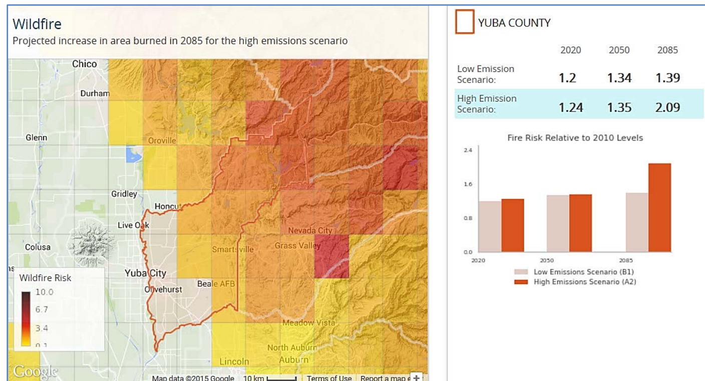
Figure 4. Relative increase in wildfire acreage in future carbon emission scenarios, Yuba County 6
