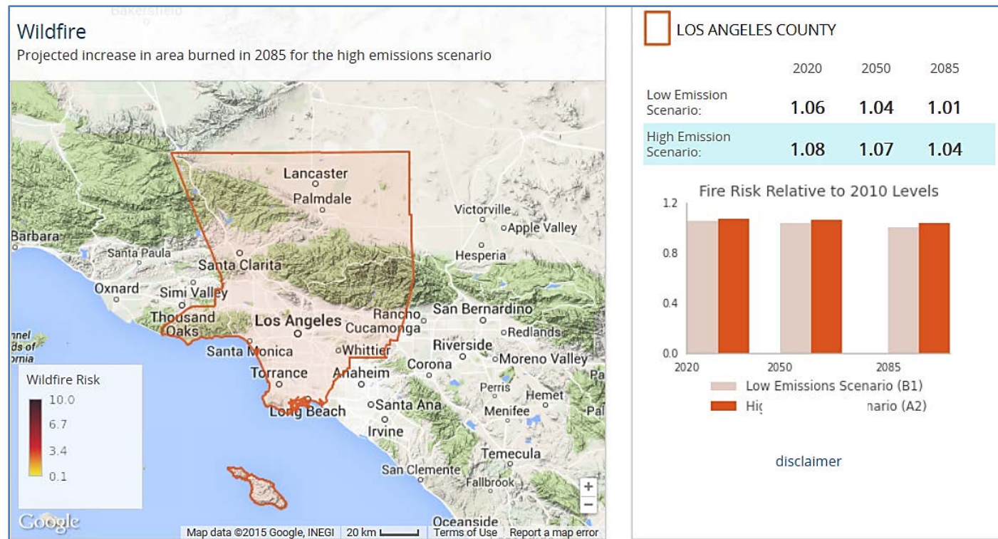
Figure 4. Relative increase in wildfire acreage in future carbon emission scenarios, Los Angeles County 6
