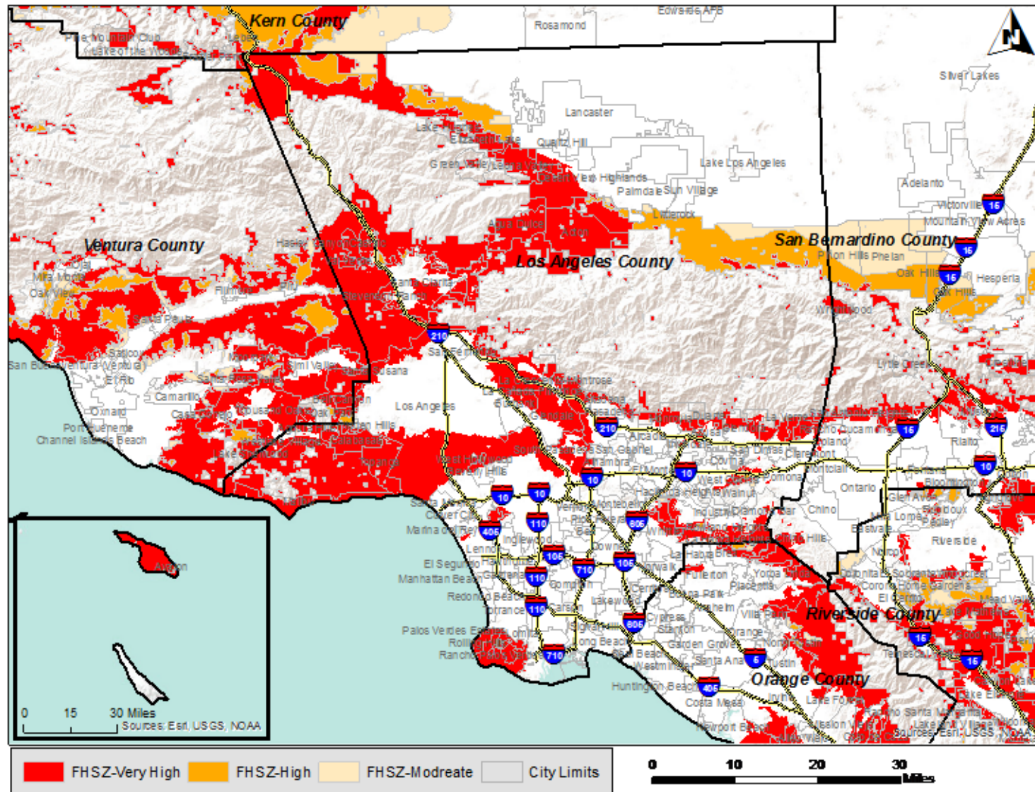
Figure 3. Current Fire Hazard Severity Zones (FHSZ), Los Angeles County, 2007 9
