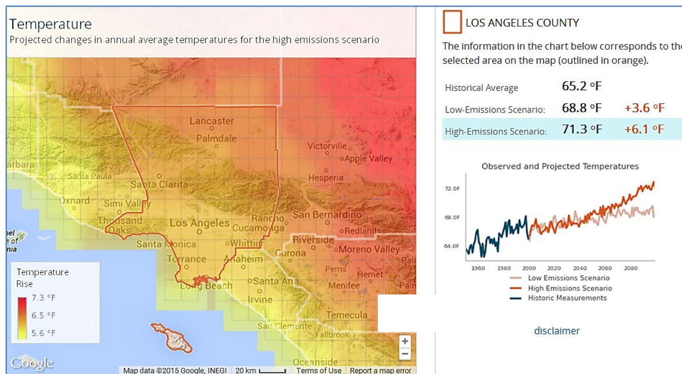
Figure 2. Projected changes in annual average temperature in future carbon emissions scenarios, Los Angeles County, 2099 6
