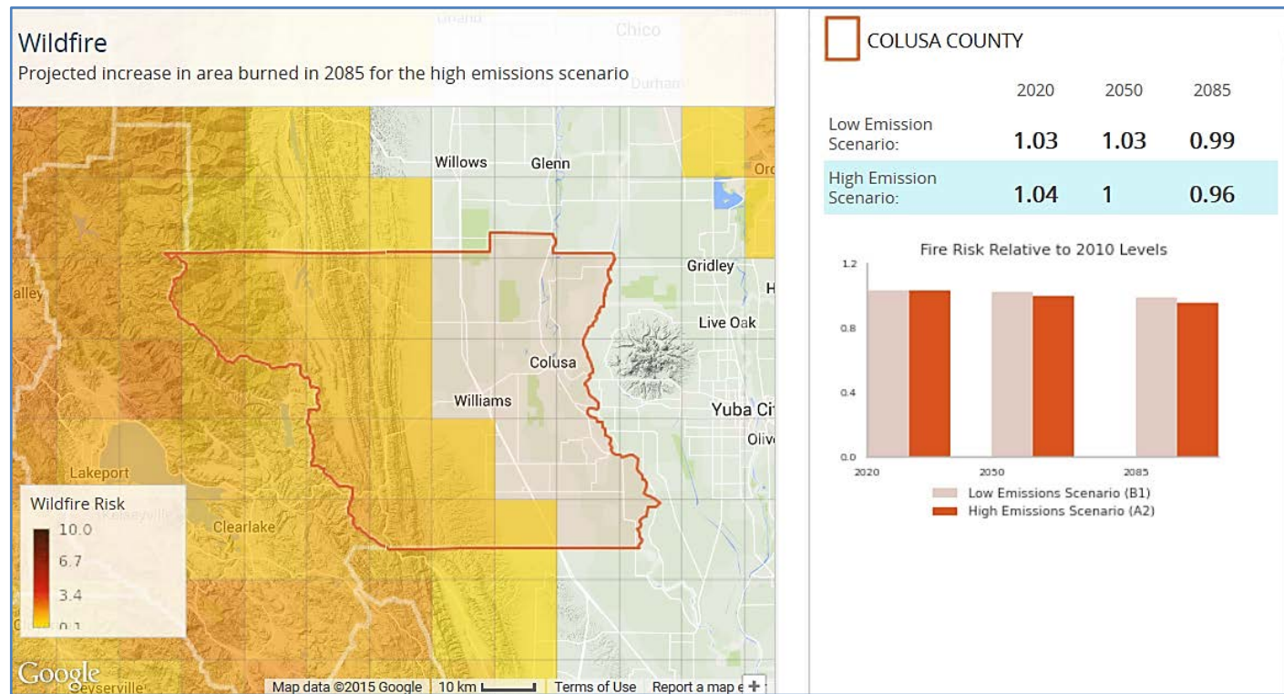
Figure 4. Relative increase in wildfire acreage in future carbon emission scenarios, Colusa County 6
