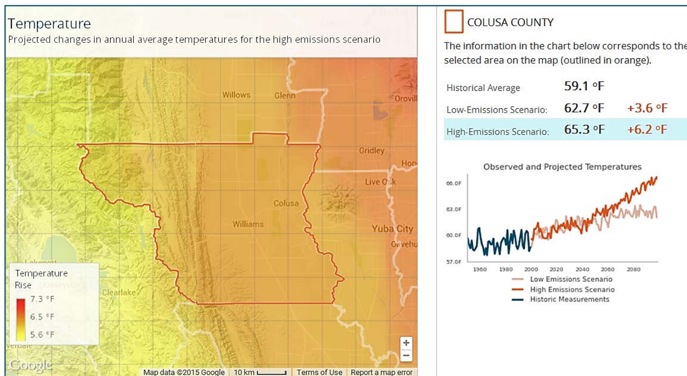
Figure 2. Projected changes in annual average temperature in future carbon emissions scenarios, Colusa County, 2099 6
