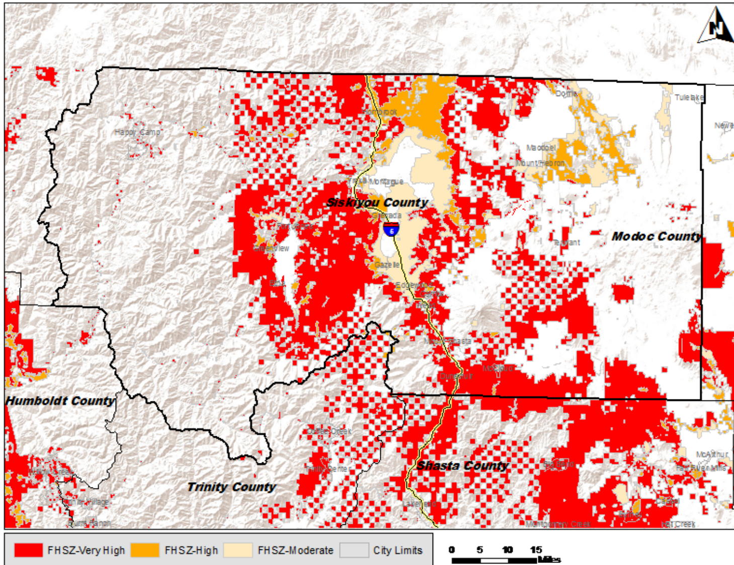
Figure 3. Current Fire Hazard Severity Zones (FHSZ), Siskiyou County, 2007 8 Note: Map includes only state and local responsibility areas.
