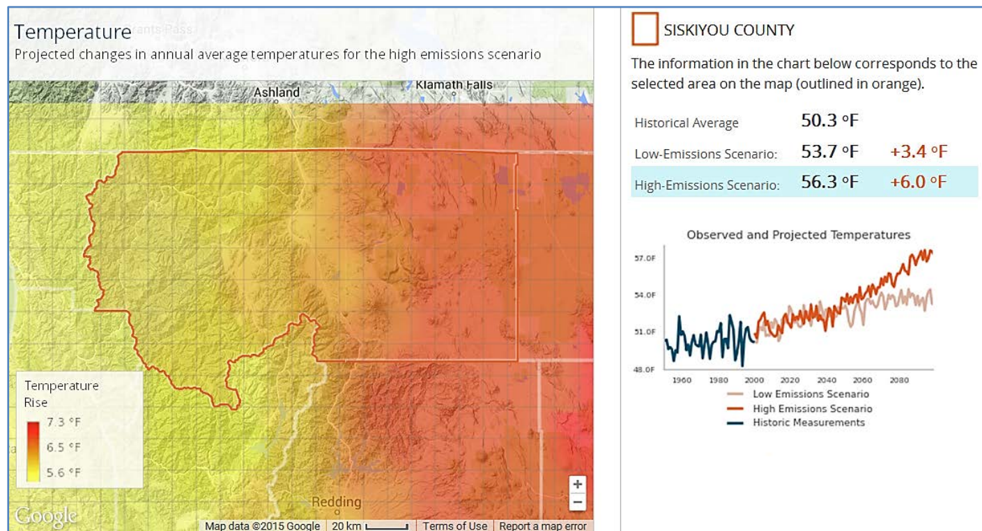
Figure 2. Projected changes in annual average temperature in future carbon emissions scenarios, Siskiyou County, 2099 6
