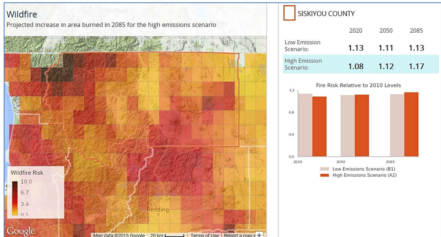
Figure 4. Relative increase in wildfire acreage in future carbon emission scenarios, Siskiyou County 6
