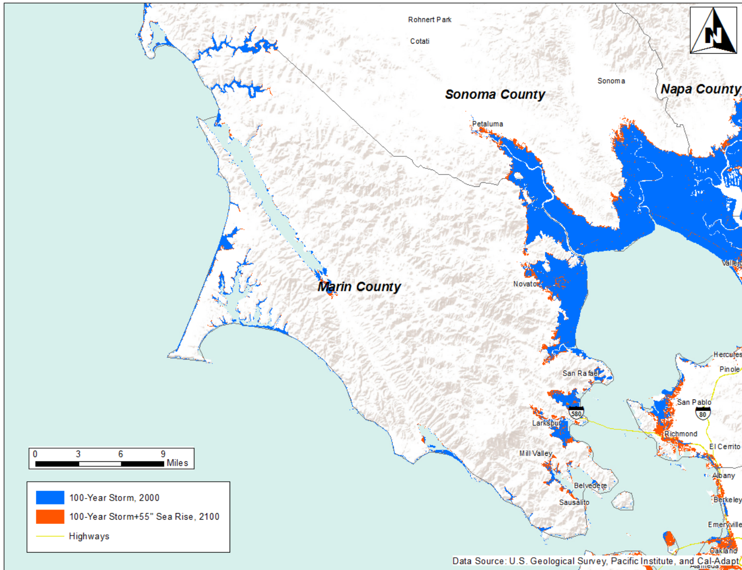
Figure 5. Baseline inundation areas for a 100-year flood (2000) and modeled scenario with additional 55 inches of sea level rise (2100), Marin County 6 Note: Current projections are 66 inches above sea level. 7
