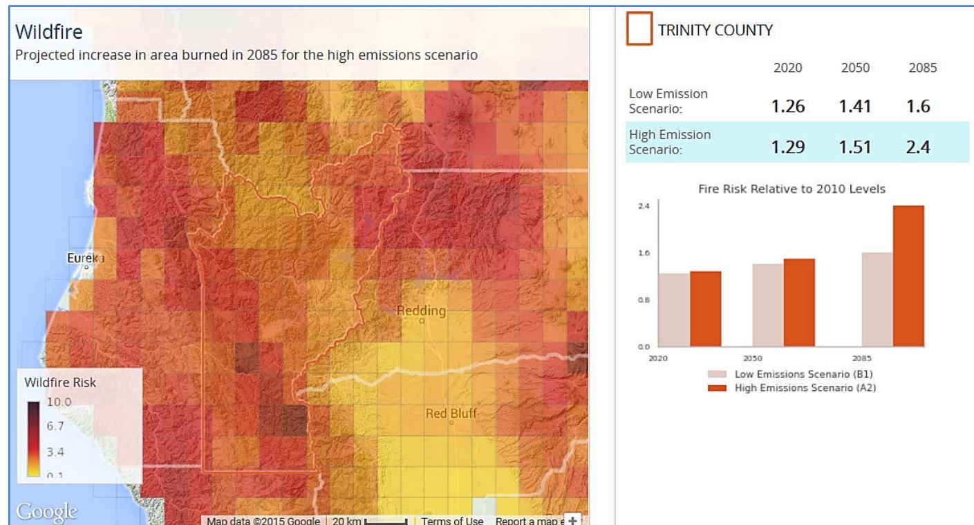
Figure 4. Relative increase in wildfire acreage in future carbon emission scenarios, Trinity County 6
