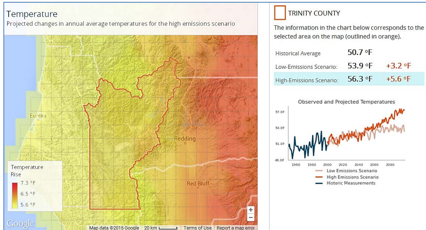
Figure 2. Projected changes in annual average temperature in future carbon emissions scenarios, Trinity County, 2099 6
