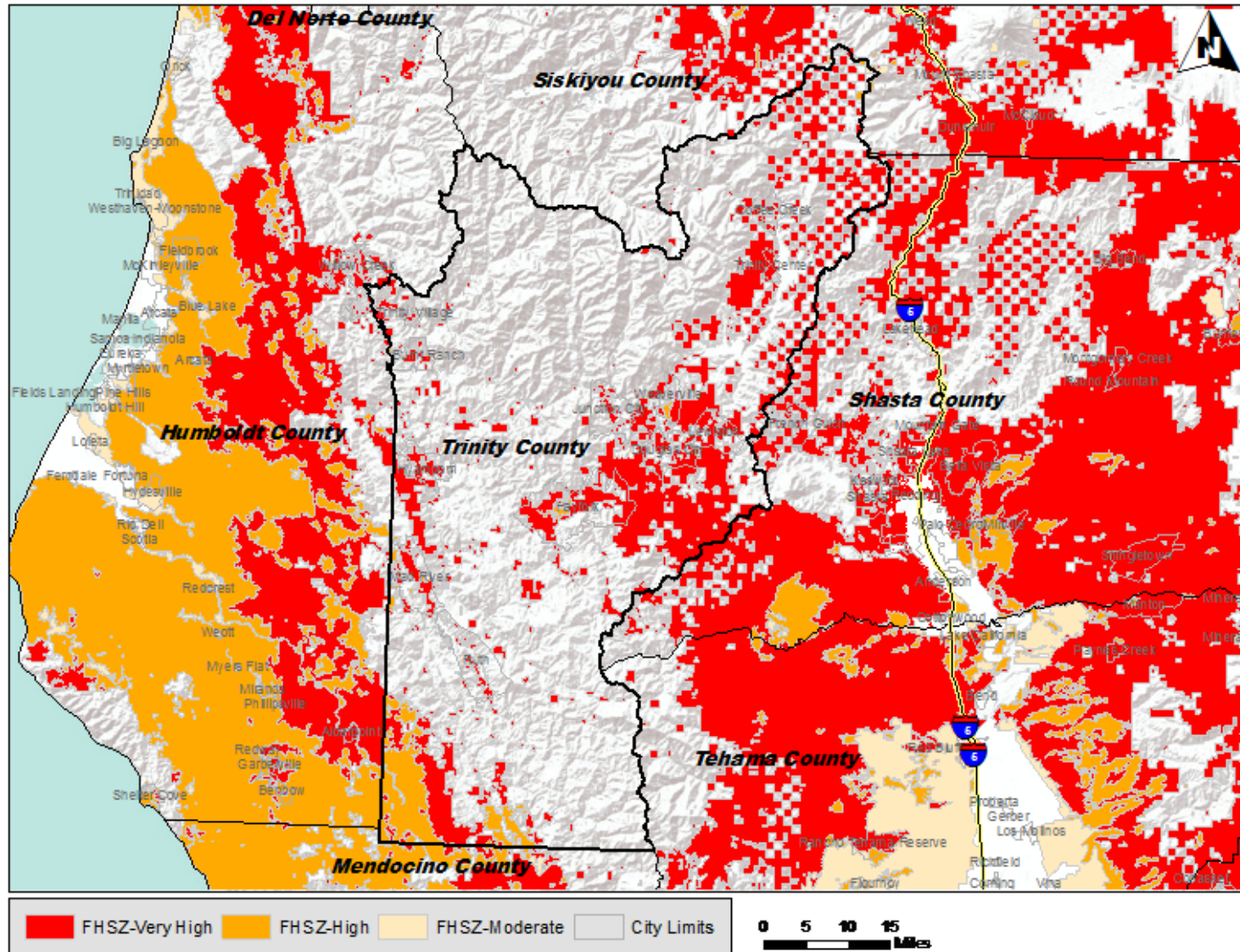
Figure 3. Current Fire Hazard Severity Zones (FHSZ), Trinity County, 2007 8 Note: Map includes only state and local responsibility areas.
