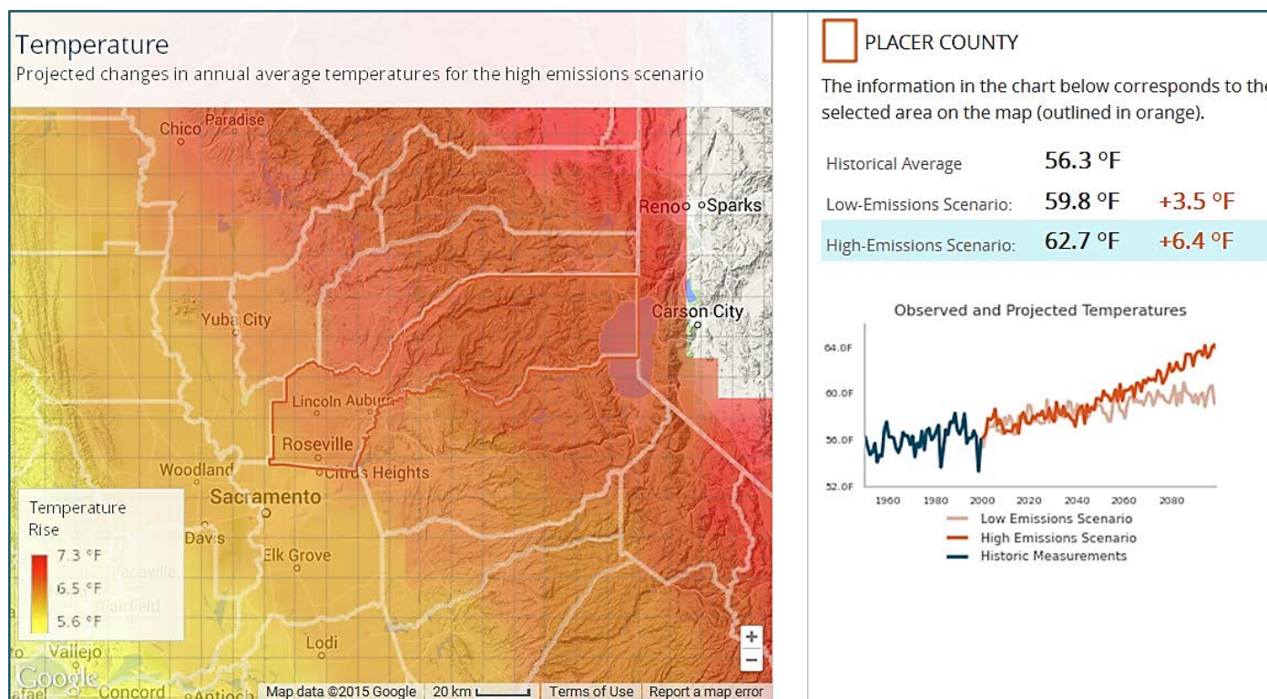
Figure 2. Projected changes in annual average temperature in future carbon emissions scenarios, Placer County, 2099 6
