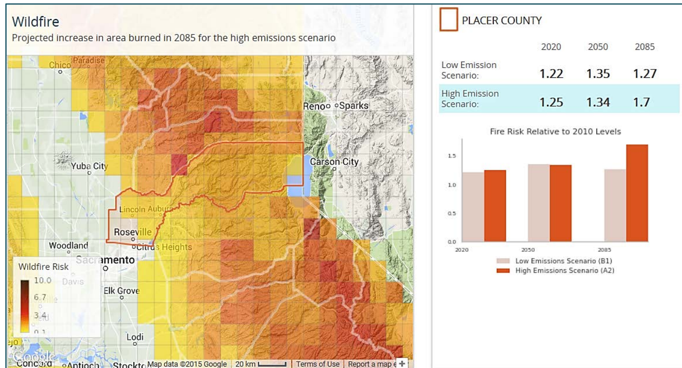
Figure 4. Relative increase in wildfire acreage in future carbon emission scenarios, Placer County 6
