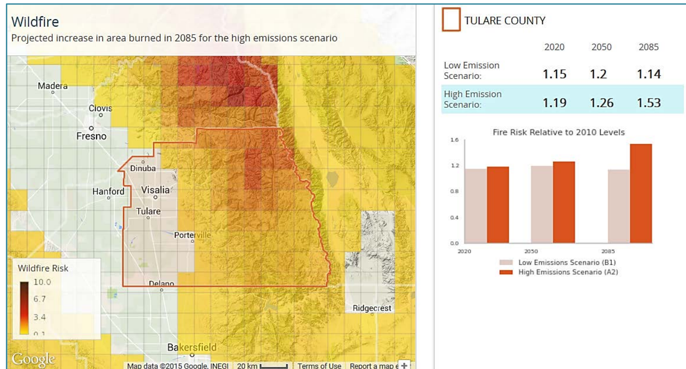
Figure 4. Relative increase in wildfire acreage in future carbon emission scenarios, Tulare County 6
