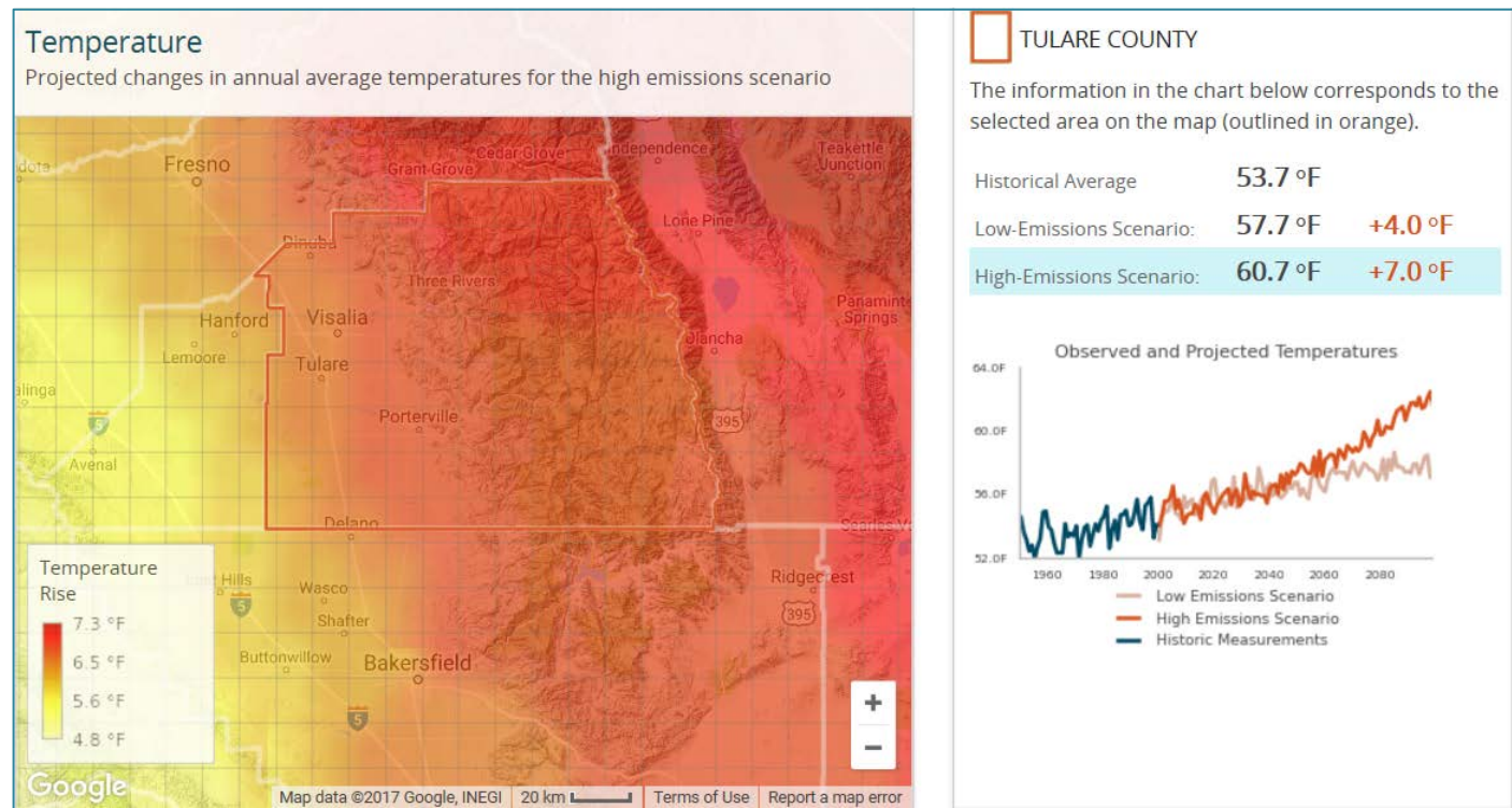
Figure 2. Projected changes in annual average temperature in future carbon emissions scenarios, Tulare County, 2099 6
