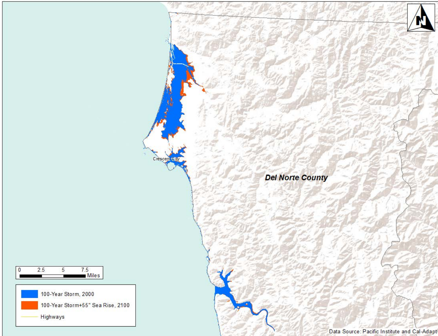
Figure 5. Baseline inundation areas for a 100-year flood (2000) and modeled scenario with additional 55 inches of sea level rise (2100), Del Norte County 6 Note: Current SLR projections are 66 inches above sea level. 7
