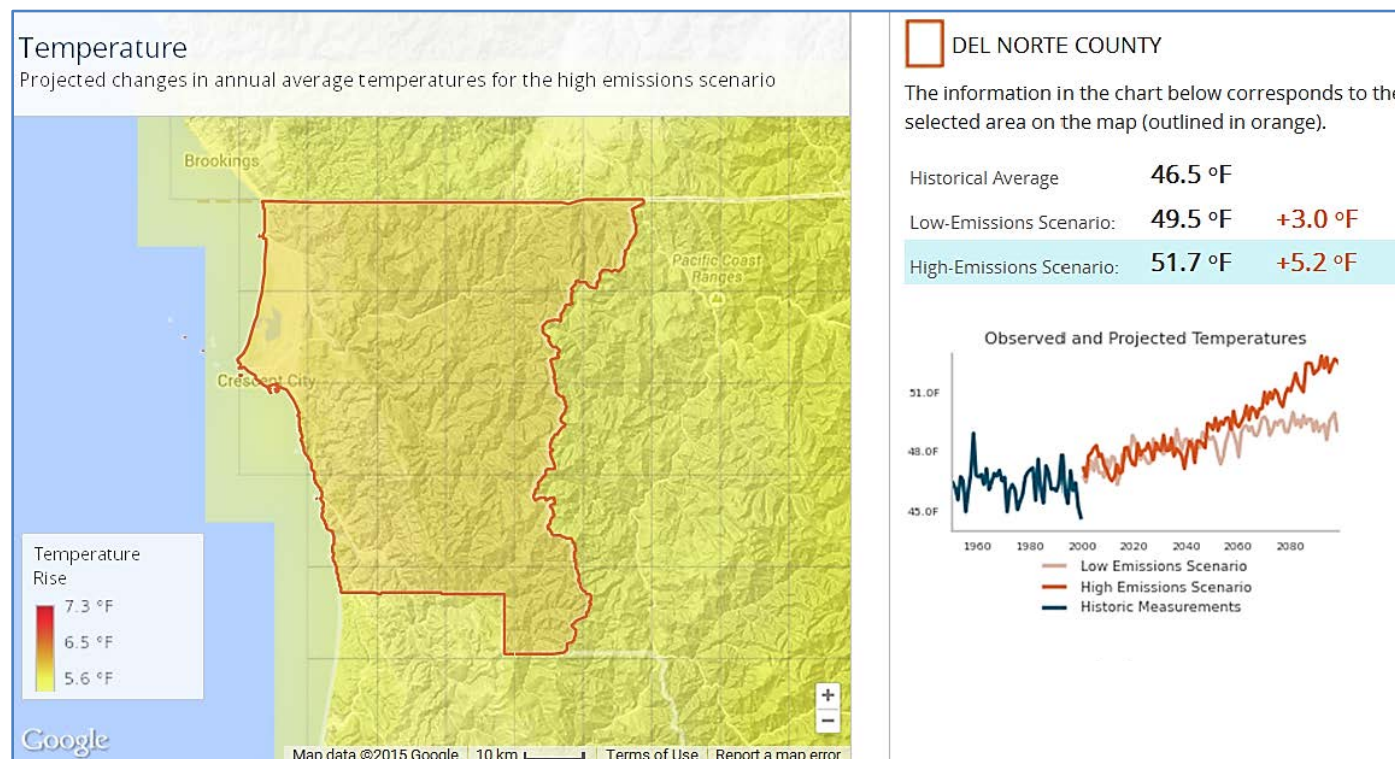
Figure 2. Projected changes in annual average temperature in future carbon emissions scenarios, Del Norte County, 2099 6
