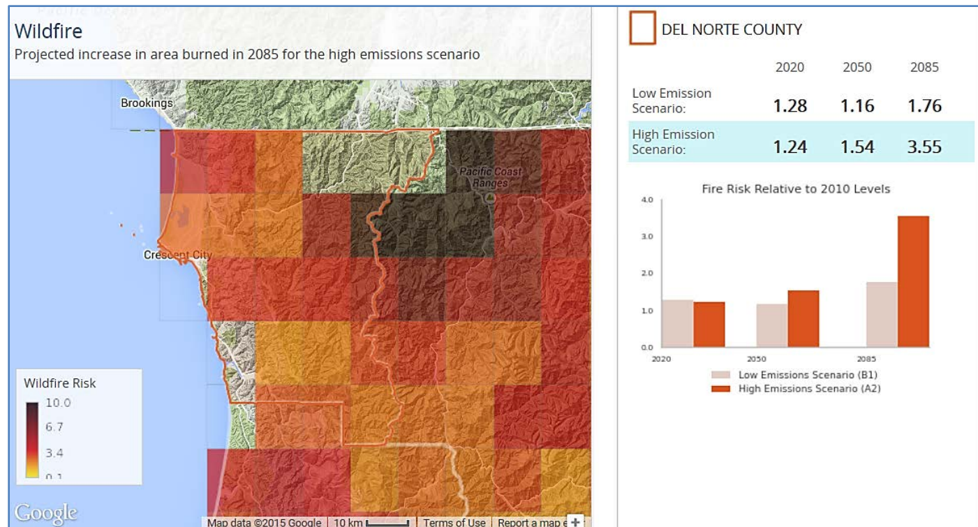
Figure 4. Relative increase in wildfire acreage in future carbon emission scenarios, Del Norte County 6
