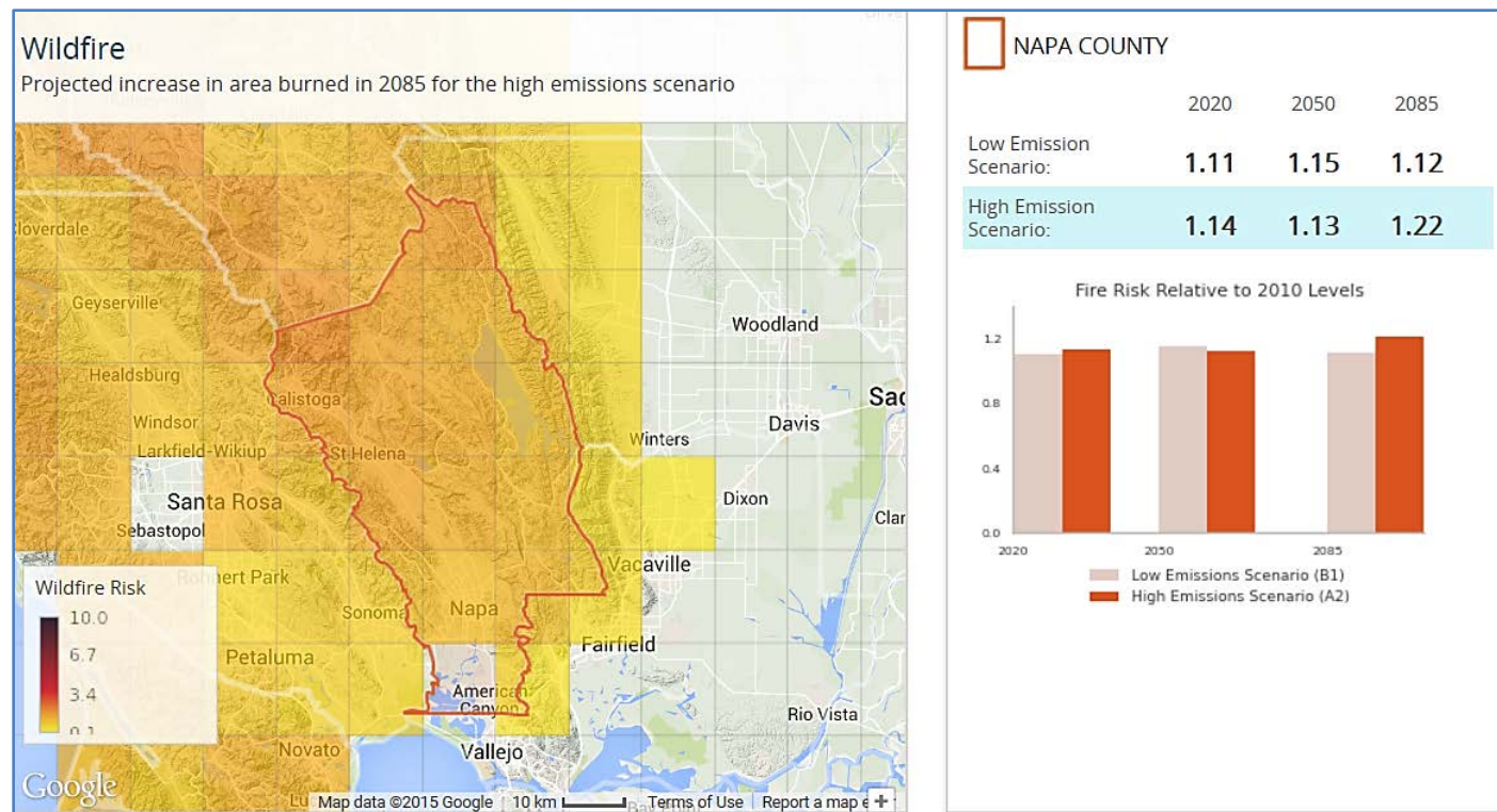
Figure 4. Relative increase in wildfire acreage in future carbon emission scenarios, Napa County 6
