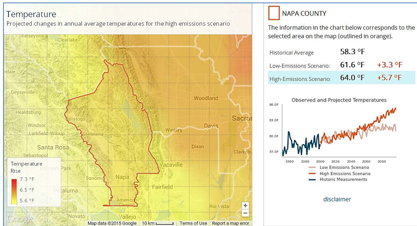
Figure 2. Projected changes in annual average temperature in future carbon emissions scenarios, Napa County, 2099 6
