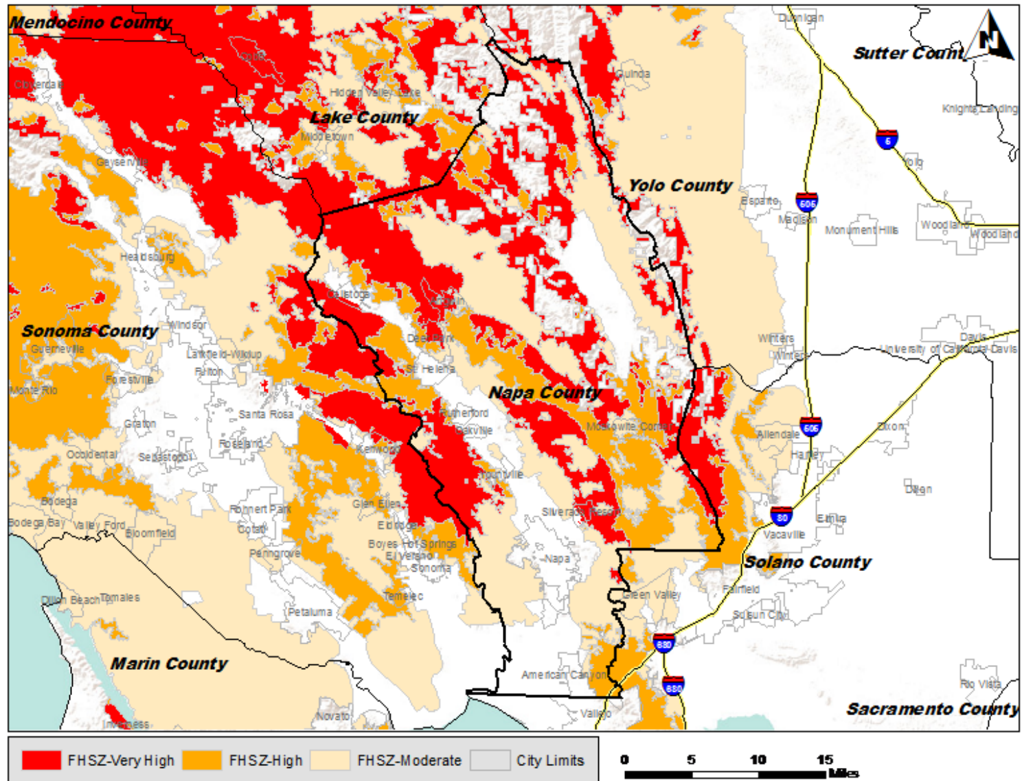
Figure 3. Current Fire Hazard Severity Zones (FHSZ), Napa County, 2007 9
